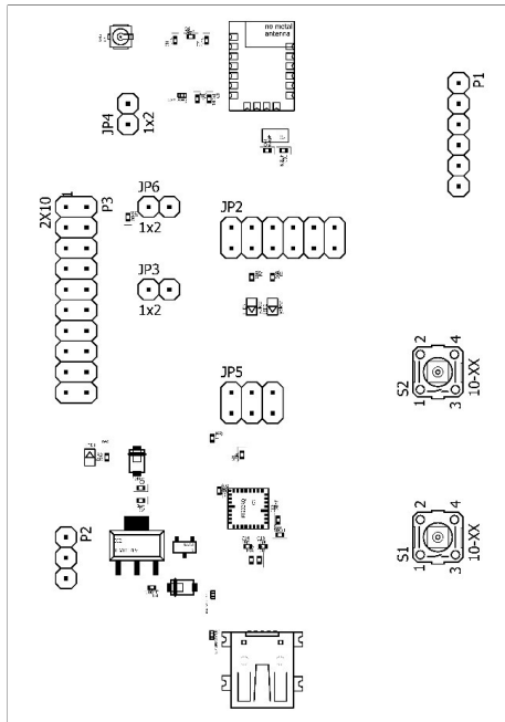
Figure 13: Assembly diagram
