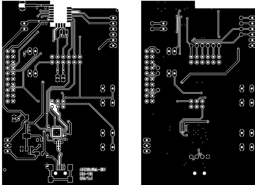
Figure 14: Top & bottom Layer
